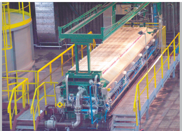
Filter press with PVDF membrane- and combination chamber plate 1200 x 1200 mm, application Metallurgy, chemistry etc.
